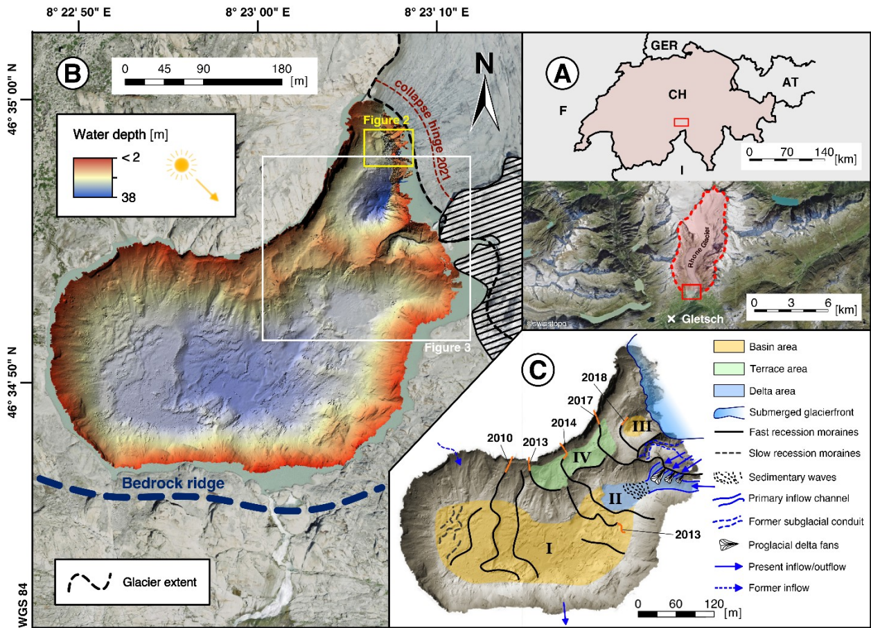
Figure 1. A: Location of the catchment area in the Central Swiss Alps. B: High-resolution bathymetric map of Rhone Lake recorded in 2021. Background map by swisstopo. Glacier extent marked by black dashed line. Striped area in the east indicates glacier covered by white blankets to prevent ice melting preserving a touristic ice cave. C: Morphological interpretation of the bathymetric dataset from 2021.
