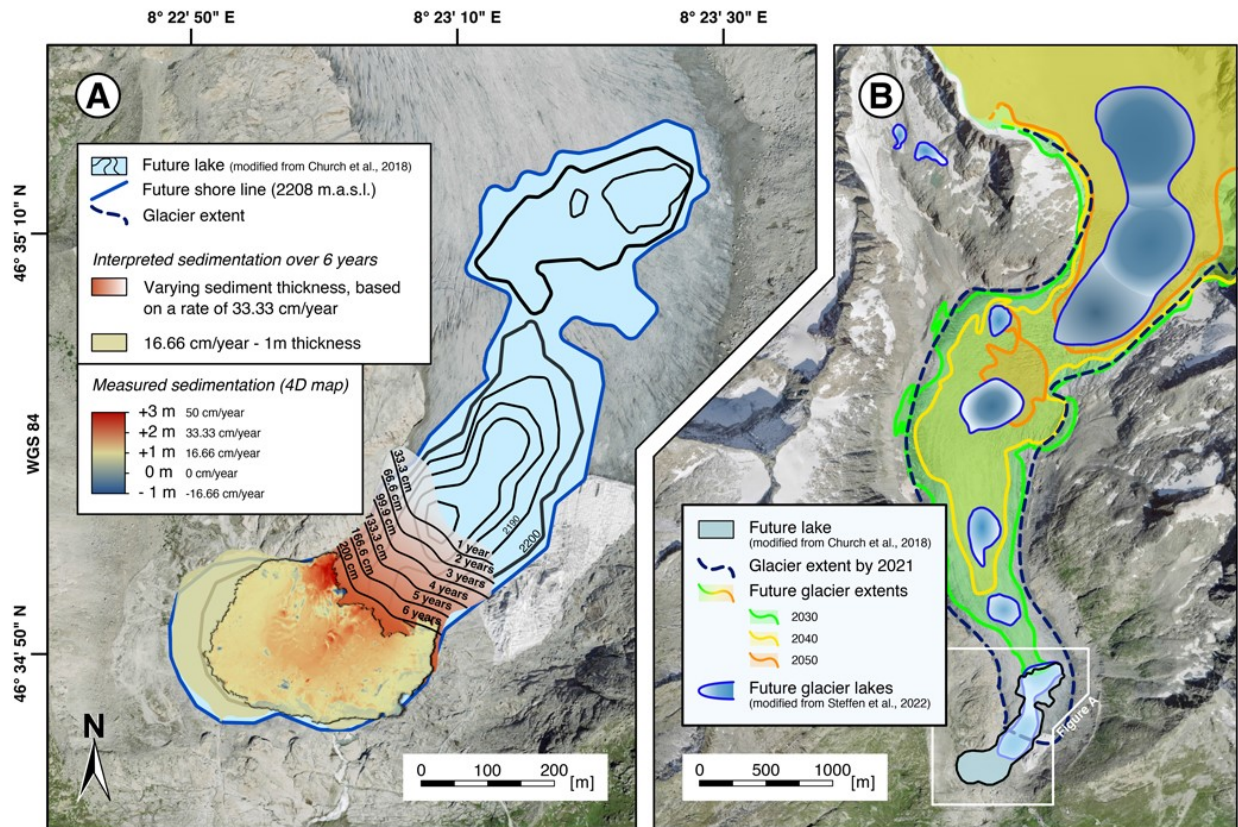
Figure 4. A: Sediment thickness over six years based on two repetitive bathymetric surveys and retreating ice tongue. Future lake, modified from Church et al. (2018). B: Future proglacial lakes at the Rhonegletscher based on calculations by swisstopo.
