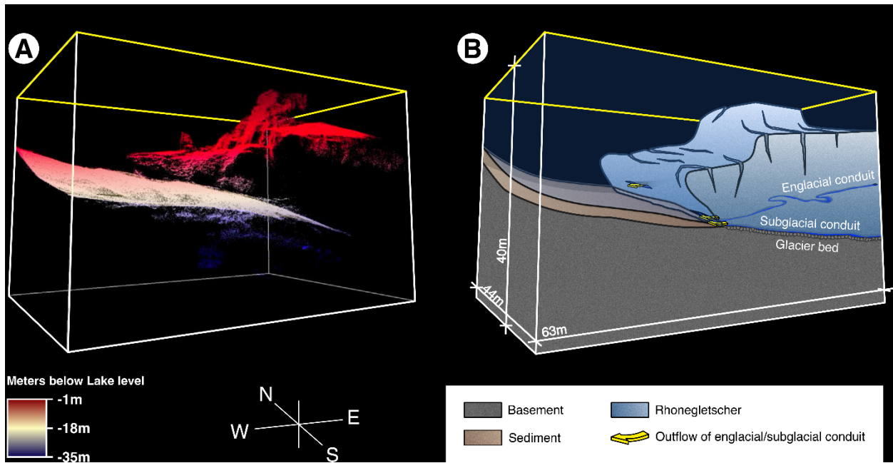
Figure 2. A: Ungridded point cloud of swath-bathymetry data of the submerged glacier front. B: 3D-interpretation of the data in Fig A. Model shows morphological features contributing to the formation of a subglacial overdeepening.
